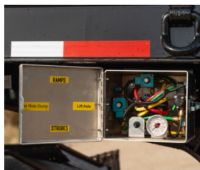
Control box located at landing gear with load scale gauge
